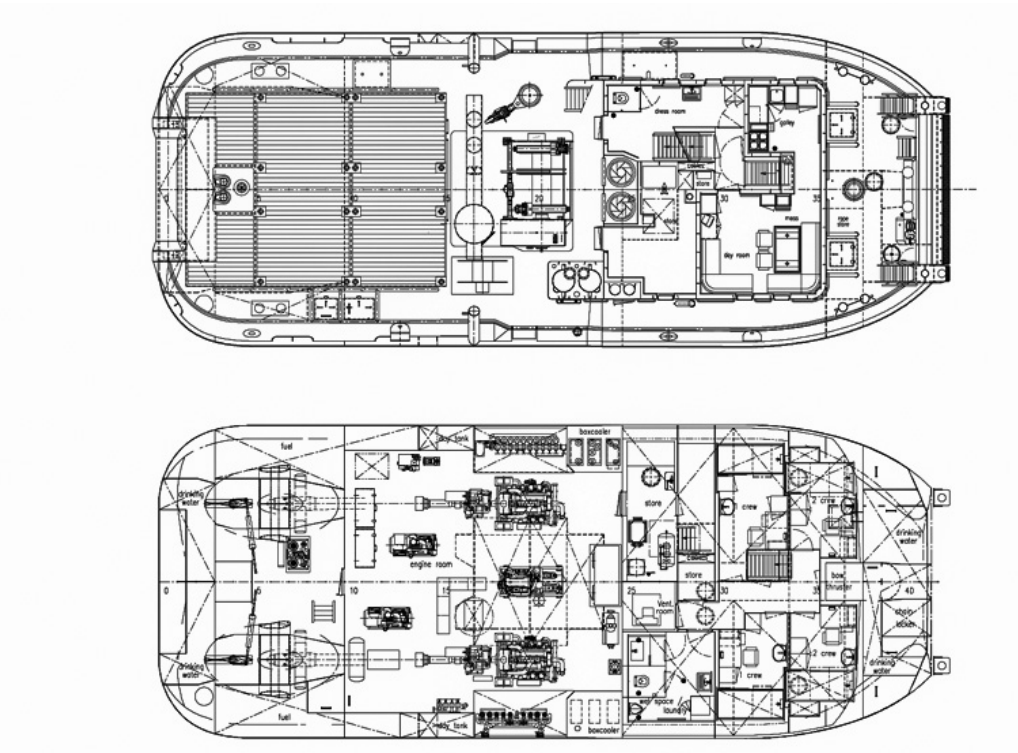
TOP VIEW DECK LEVEL
