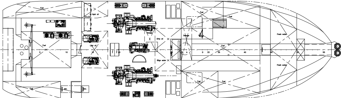
Below maindeck
